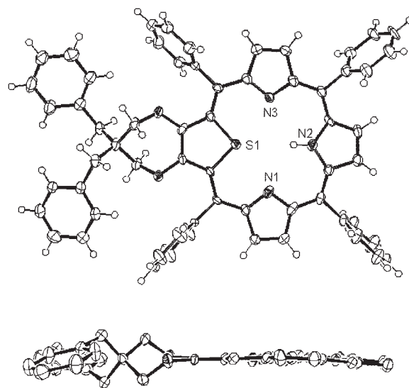
Fig. 4. ORTEP drawing for 6 (top, plane view; bottom, side view). Crystal data: C 64.5 H 49 N 3 O 2 S, purple needles, triclinic, space group = P 1, a = 9.6630(11), b = 14.6111(16), c = 18.876(2) Å, V = 2438.1(5) Å 3 , Z = 2, density = 1.2667 g/cm 3 , T = 293(2) K, F (000) = 978, R = 0.0691, wR 2 = 0.2417.
