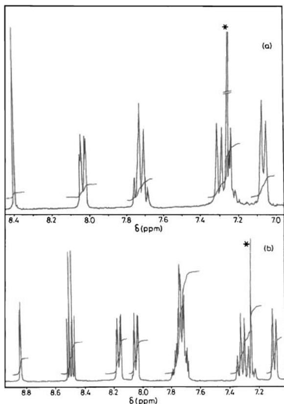
Fig. 2. 1 H NMR of (a) 3 and (b) 6 recorded in CDCl 3 .
