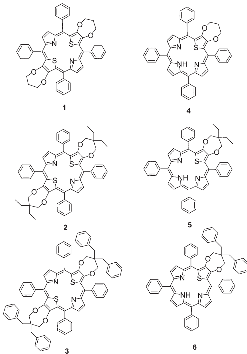
Fig. 1. Structures of \beta -thiophene substituted thiaporphyrins 1–6.
