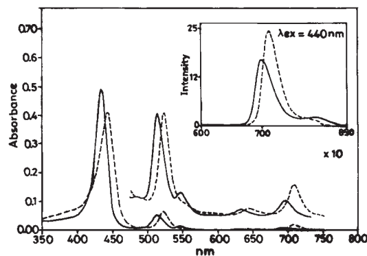
Fig. 3. Absorption and emission (inset) spectra, recorded in toluene, for S 2 TPP (—) and 3 (---).
